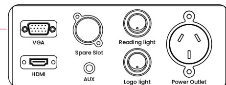
Standard Upper input panel for POD-4
